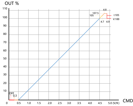
Optional edition CMD VS Output Curve(0~5V)
