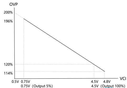
VCI VS OVP Curve
